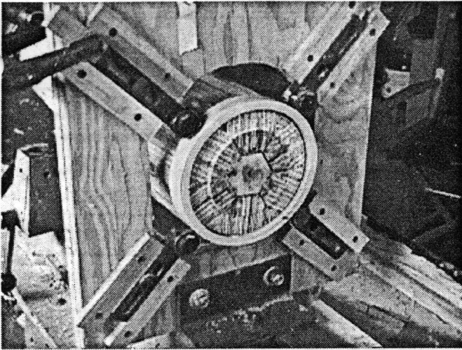
Wally's steady rest. Ball bearings run against ring cut from PVC pipe to reduce noise. Note Microlam segments.
